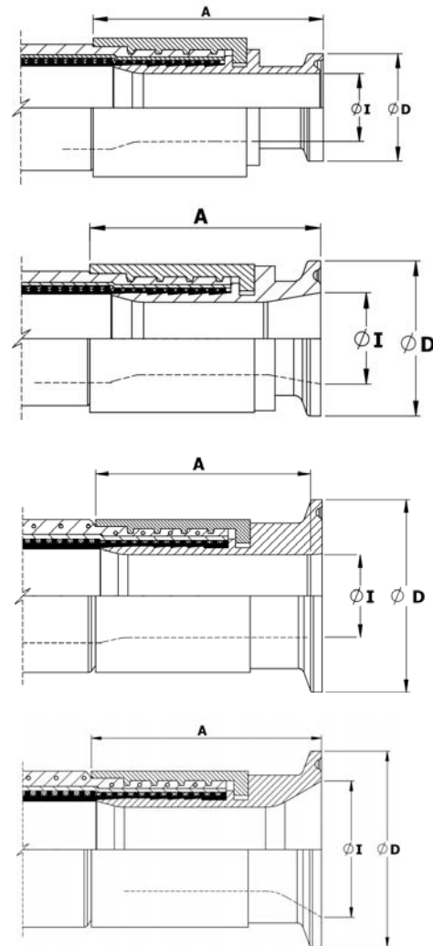
Mini-Sanitary Triclover Fittings
